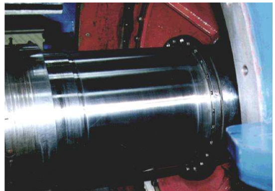
A 533 mm \varnothing Turbine Journal AFTER Machining and Polishing
